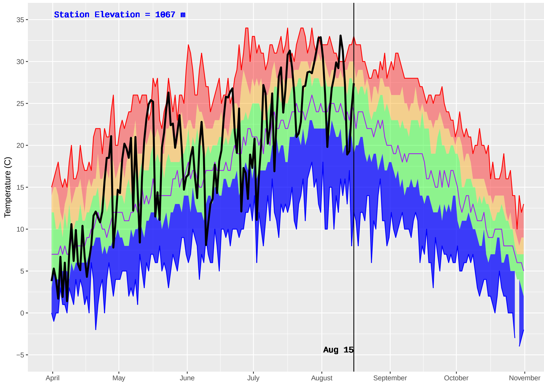
MCCUDDY (334) : Historical (1984–2016) and Current (2018) Daily Temperature
