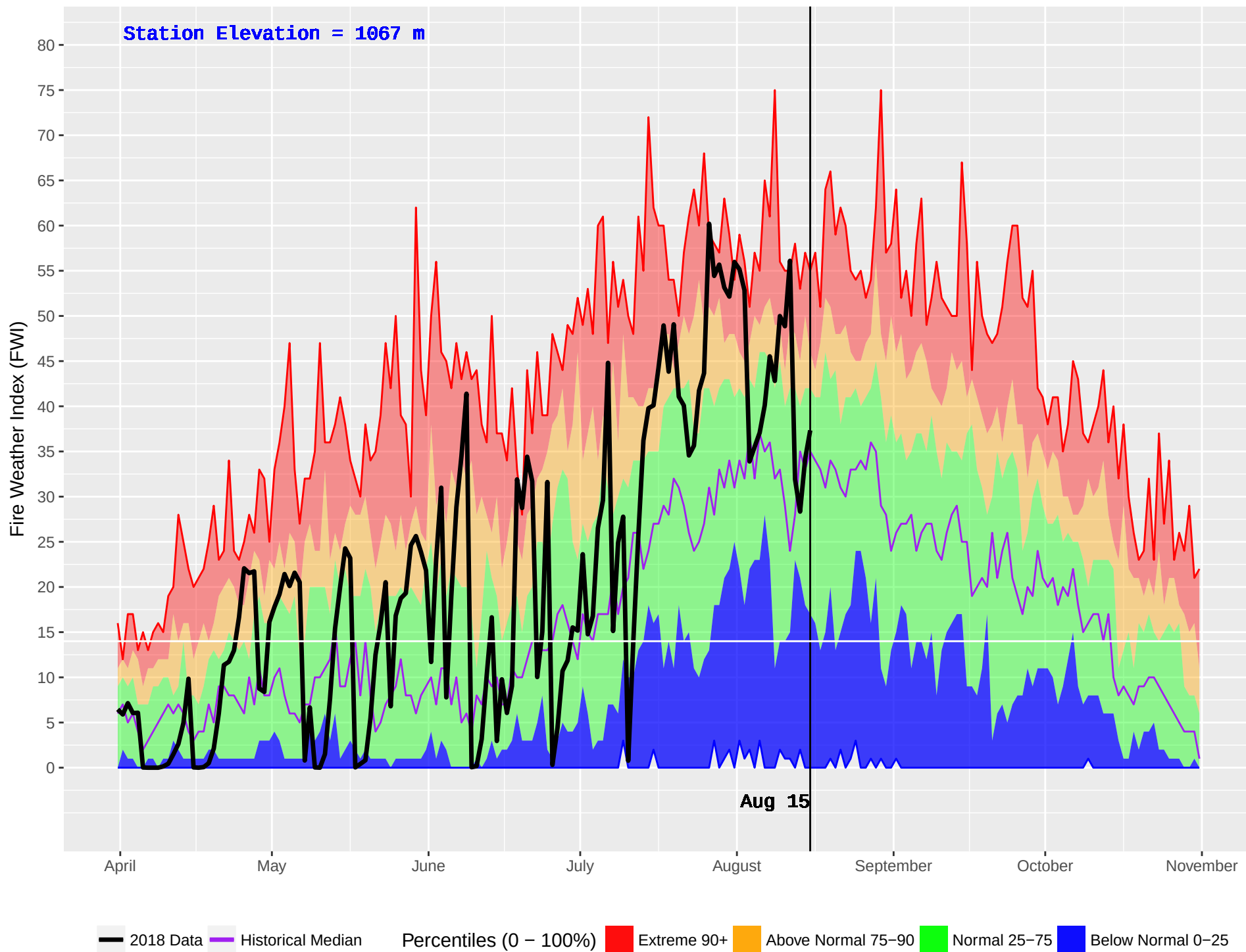
MCCUDDY (334) : Historical (1984–2016) and Current (2018) Daily Fire Weather Index (FWI)
