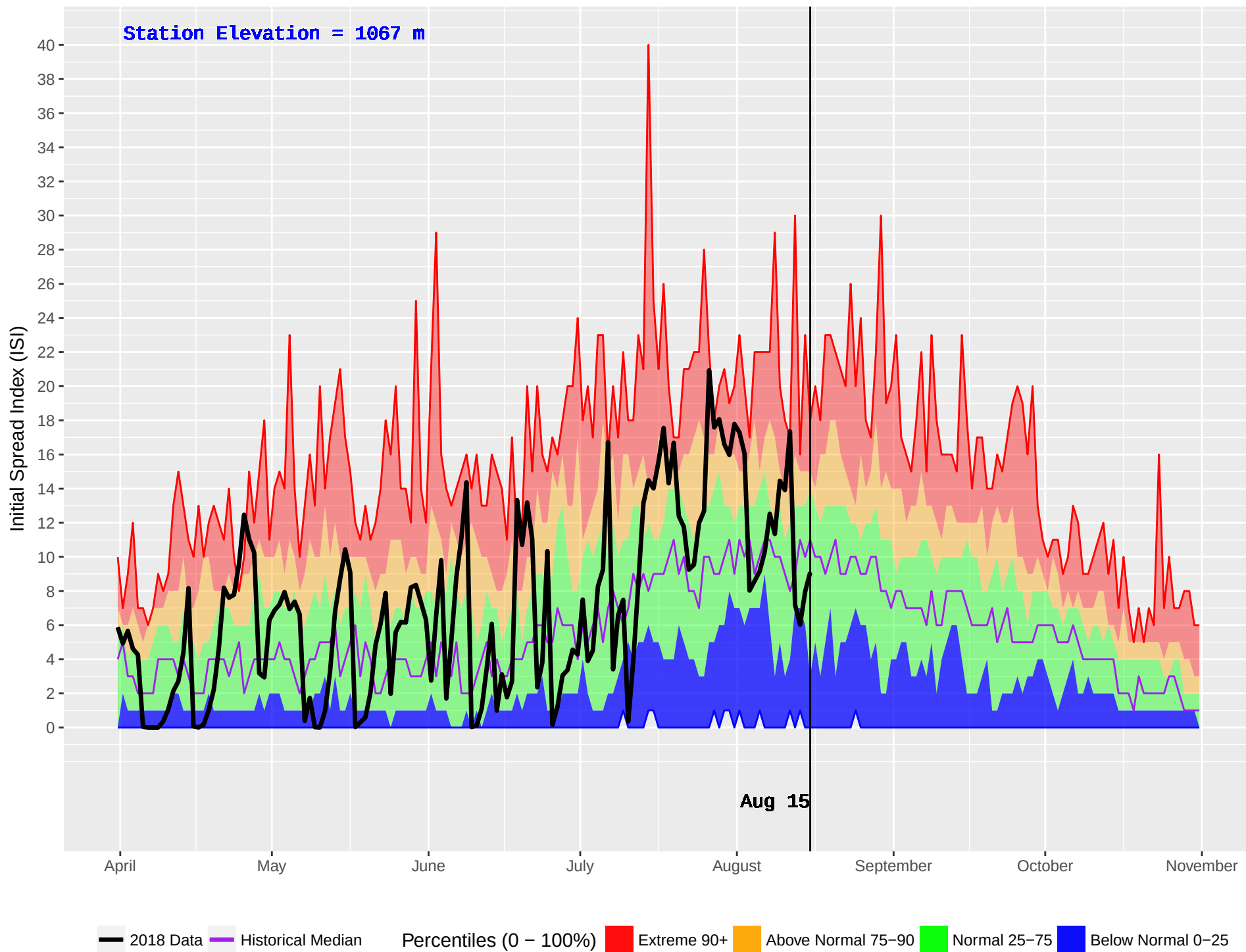
MCCUDDY (334) : Historical (1984–2016) and Current (2018) Daily Initial Spread Index (ISI)
