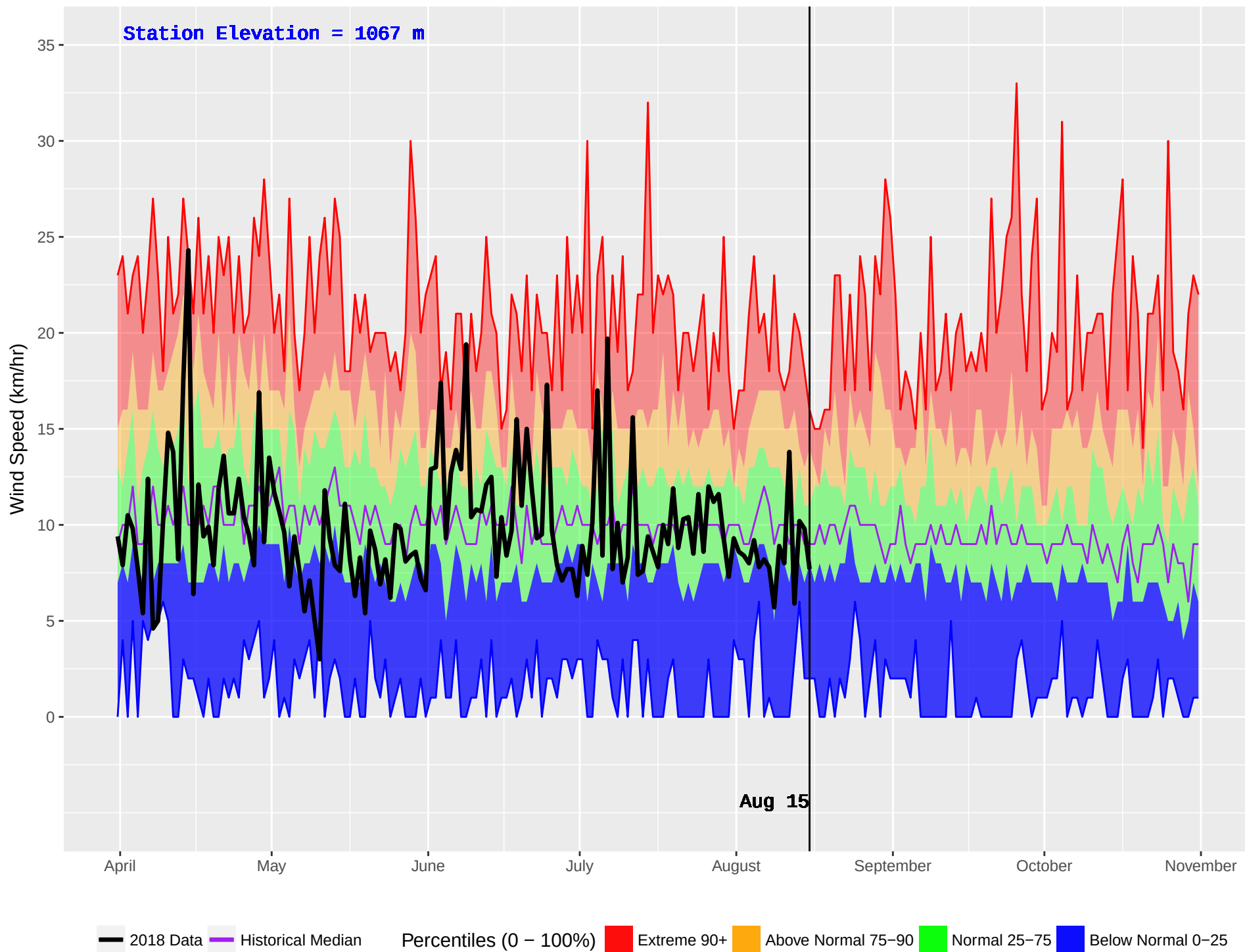
MCCUDDY (334) : Historical (1984–2016) and Current (2018) Daily Wind Speed
