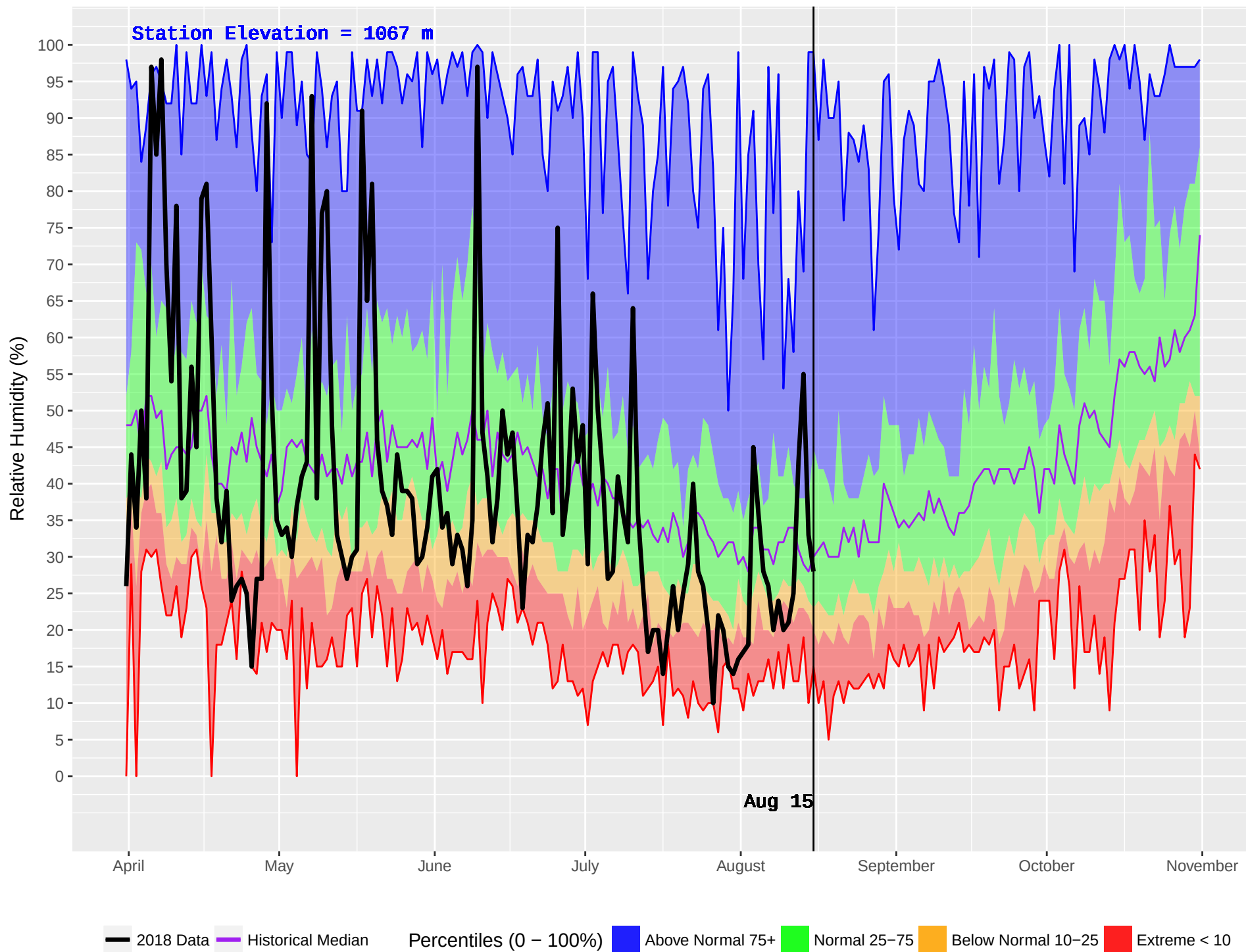
MCCUDDY (334) : Historical (1984–2016) and Current (2018) Daily Relative Humidity
